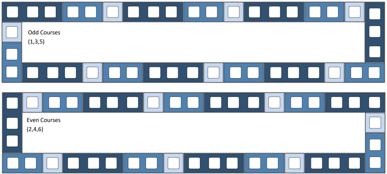
6 courses tall
