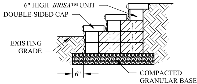
CROSS SECTION - FILL SCENARIO
