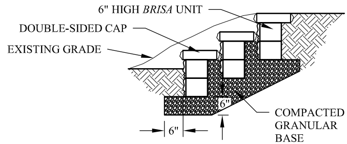
CROSS SECTION - CUT SCENARIO
