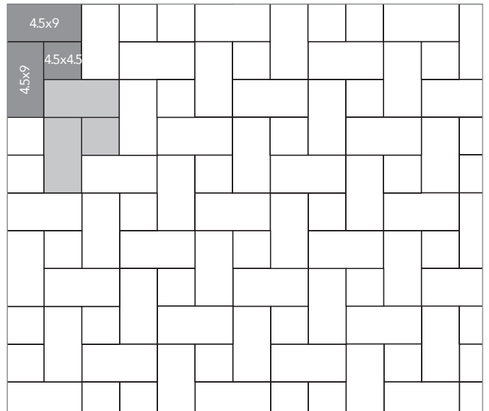
Pinwheel 20% 4.5x4.5 and 80% 4.5x9
