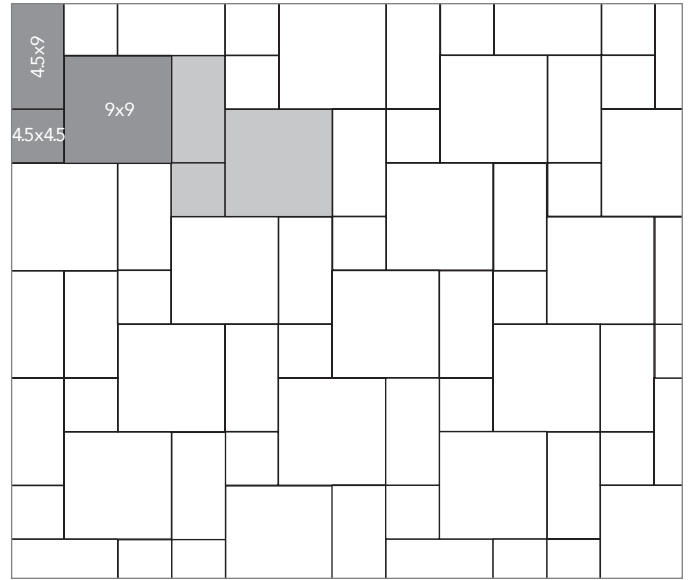
3 Piece #7 14% 4.5x4.5, 29% 4.5x9 and 57% 9x9
