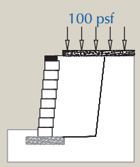
Case B Level, 100 psf Surcharge
