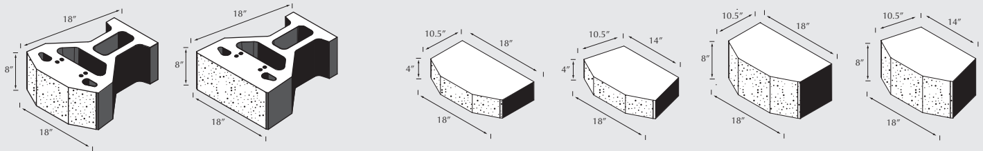
Straight Face Weight: 113 lbs Face area/unit: 1 sf Units/pallet: 30
