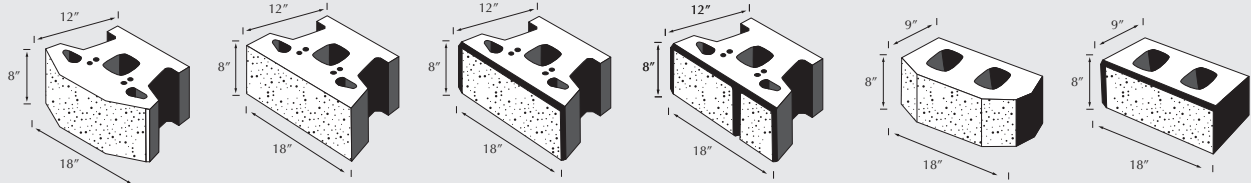
Tri-Plane Face Weight: 75 lbs Face area/unit: 1 sf Units/pallet: 45
