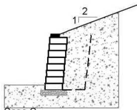
Case C Sloping, No Surcharge
