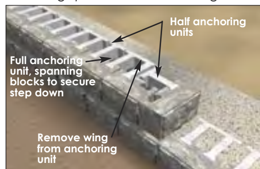
Install the half of an anchoring unit.
