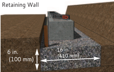
Retaining Wall
